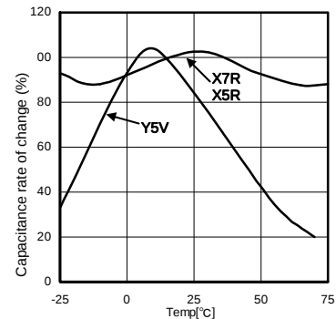
Fig. 28 Capacitance vs Temperature (X5R, X7R, Y5V)
