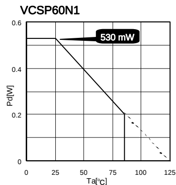
Fig. 25 VCSP60N1 Power Dissipation/Power Dissipation Reduction (Example)
