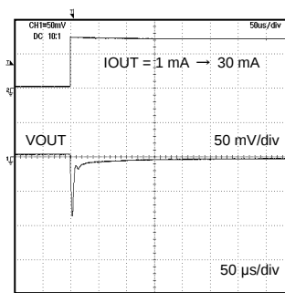
Fig. 20 Load Response (Co = 1.0 μF) (BH33RB1WGUT)
