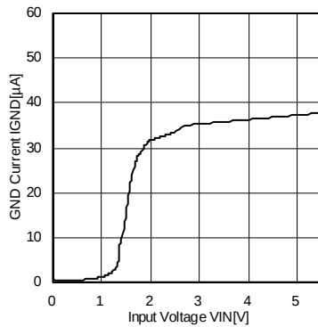
Fig. 4 GND Current vs Input Voltage (BH15RB1WGUT)
