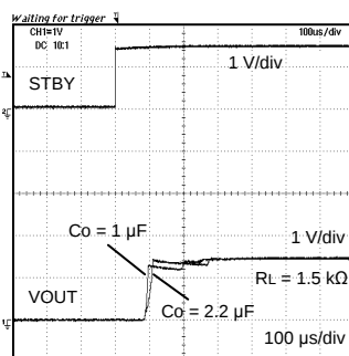
Fig. 21 Output Voltage Rise Time (BH15RB1WGUT)
