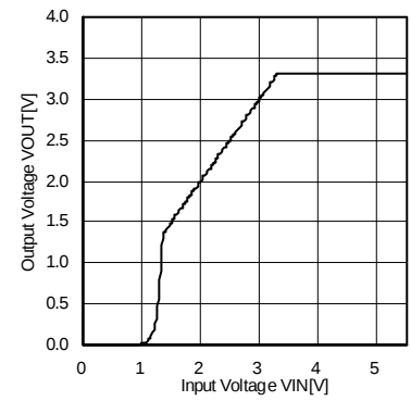
Fig. 3 Output Voltage vs Input Voltage (BH33RB1WGUT)
